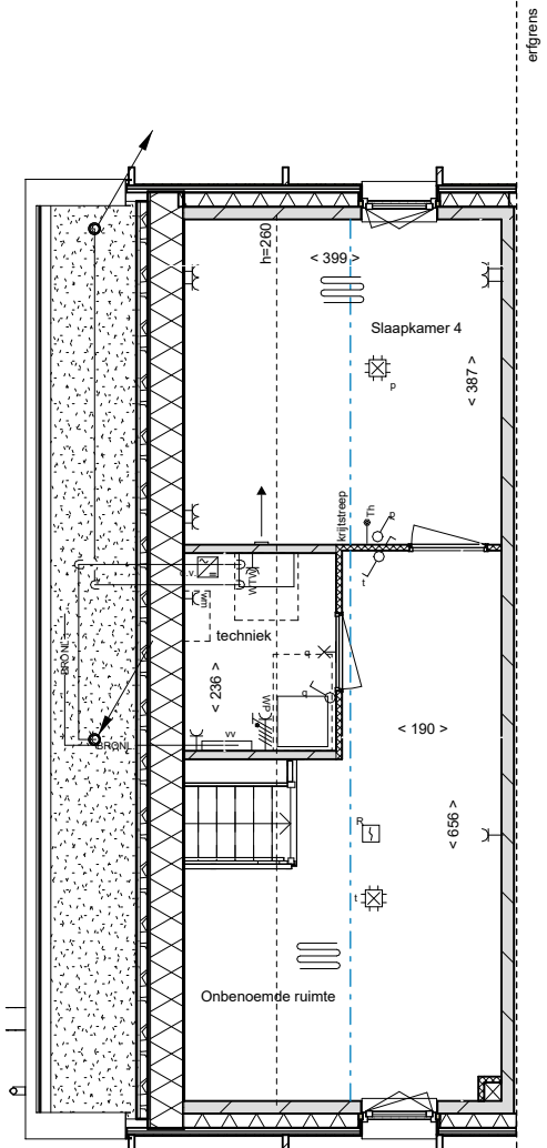
zolder
